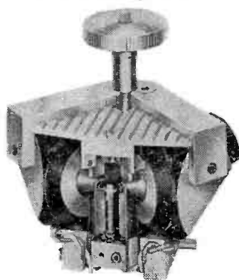
S-1 Cutting Head
